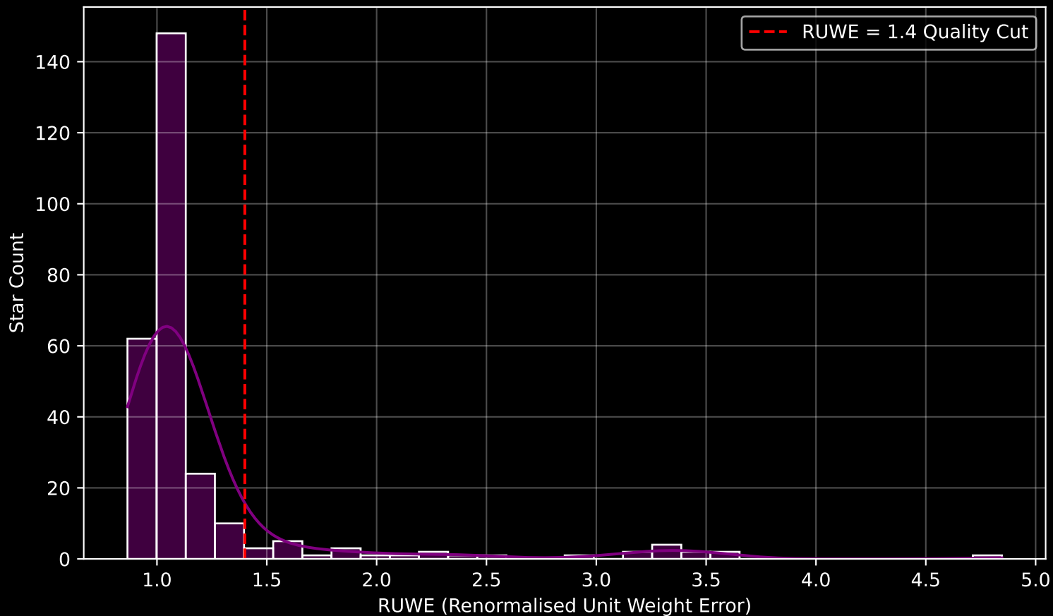
GALAH DR4 Field [1012] RUWE Distribution (n= 274)
