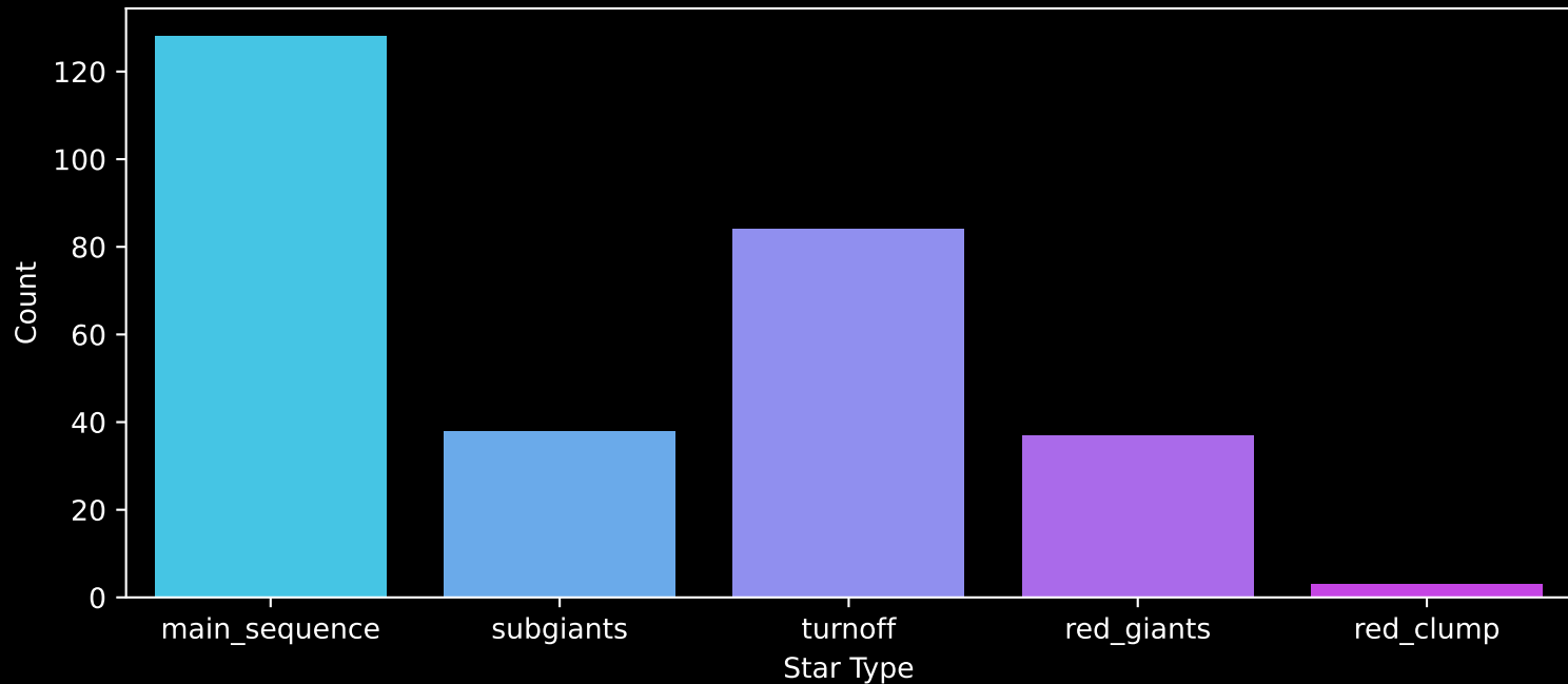
GALAH DR4 Field: [1012] Count plot of Star Type
