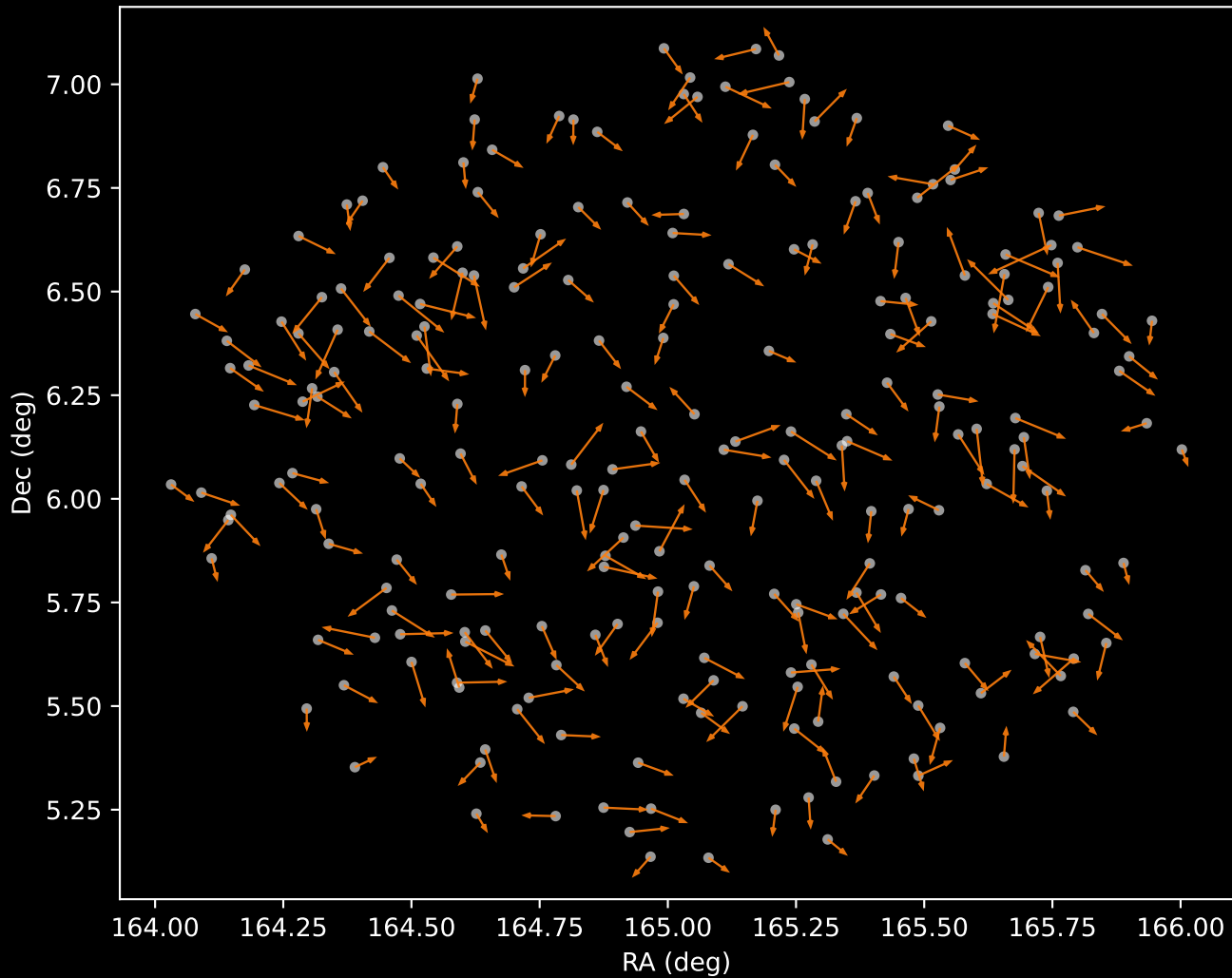
GALAH DR4 Cluster 2 Proper Motion Vectors (n=229)
