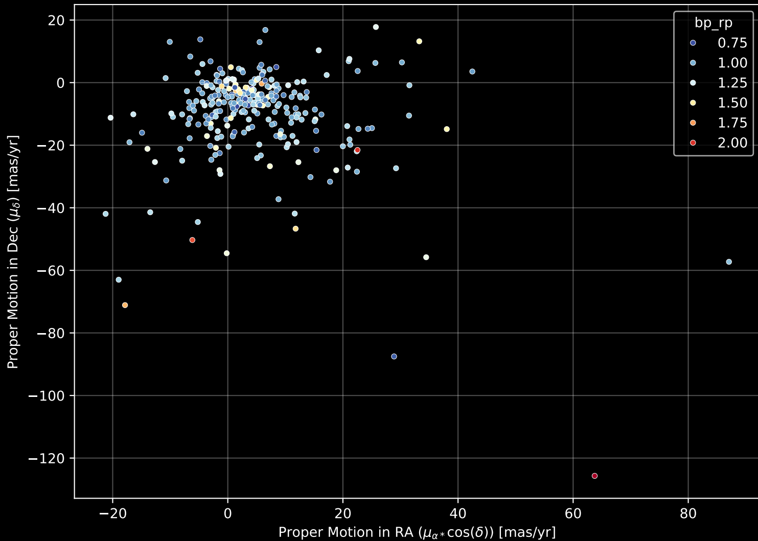
GALAH DR4 Field: [1012] Proper Motion Diagram (n= 290)
